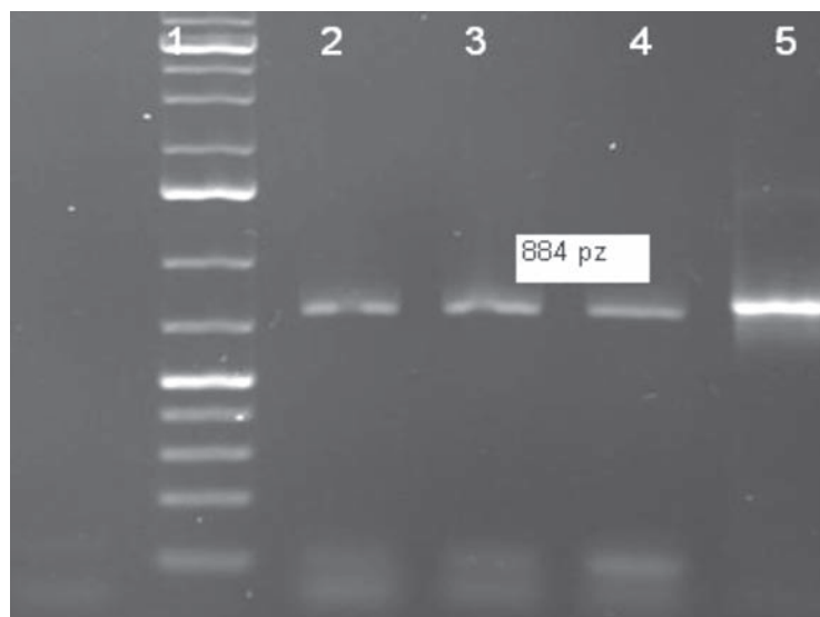
Photo 1. Separation of PCR products in 1.5% agarose gel of the uspA gene fragment (884 bp) specific for Escherichia coli
